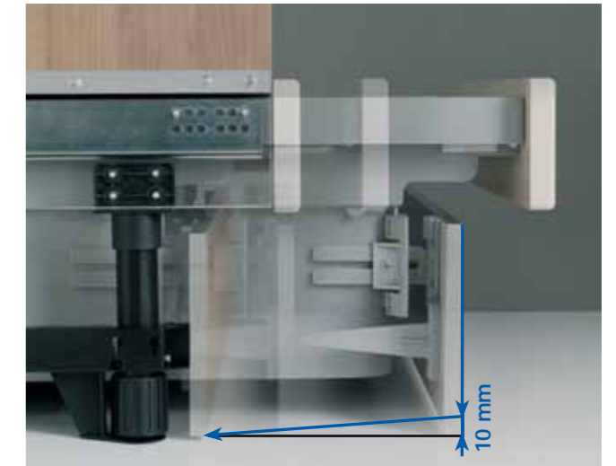
Mehr Komfort durch Blenden-Lift-Beschlag. More Convenience through panel-lift fittings.
